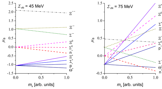
FIG. 2 (color online). Dependence of magnetic moments on m_s for \Sigma_{\pi N} = 45 and 75 MeV.
